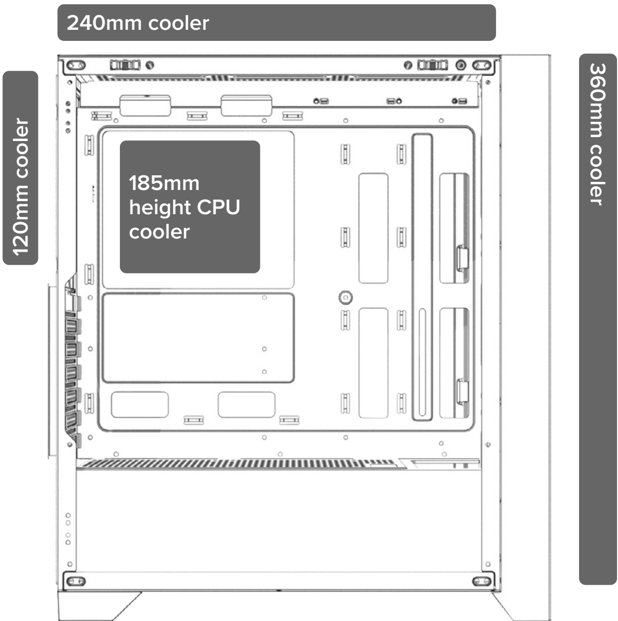
Radiator and Heatsink installation options
