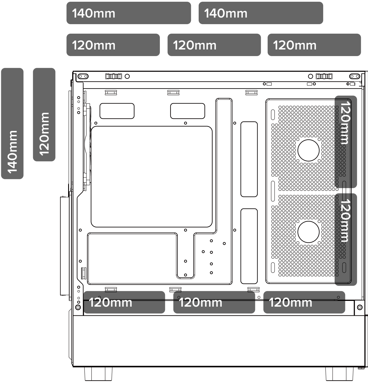
Fans installation options
