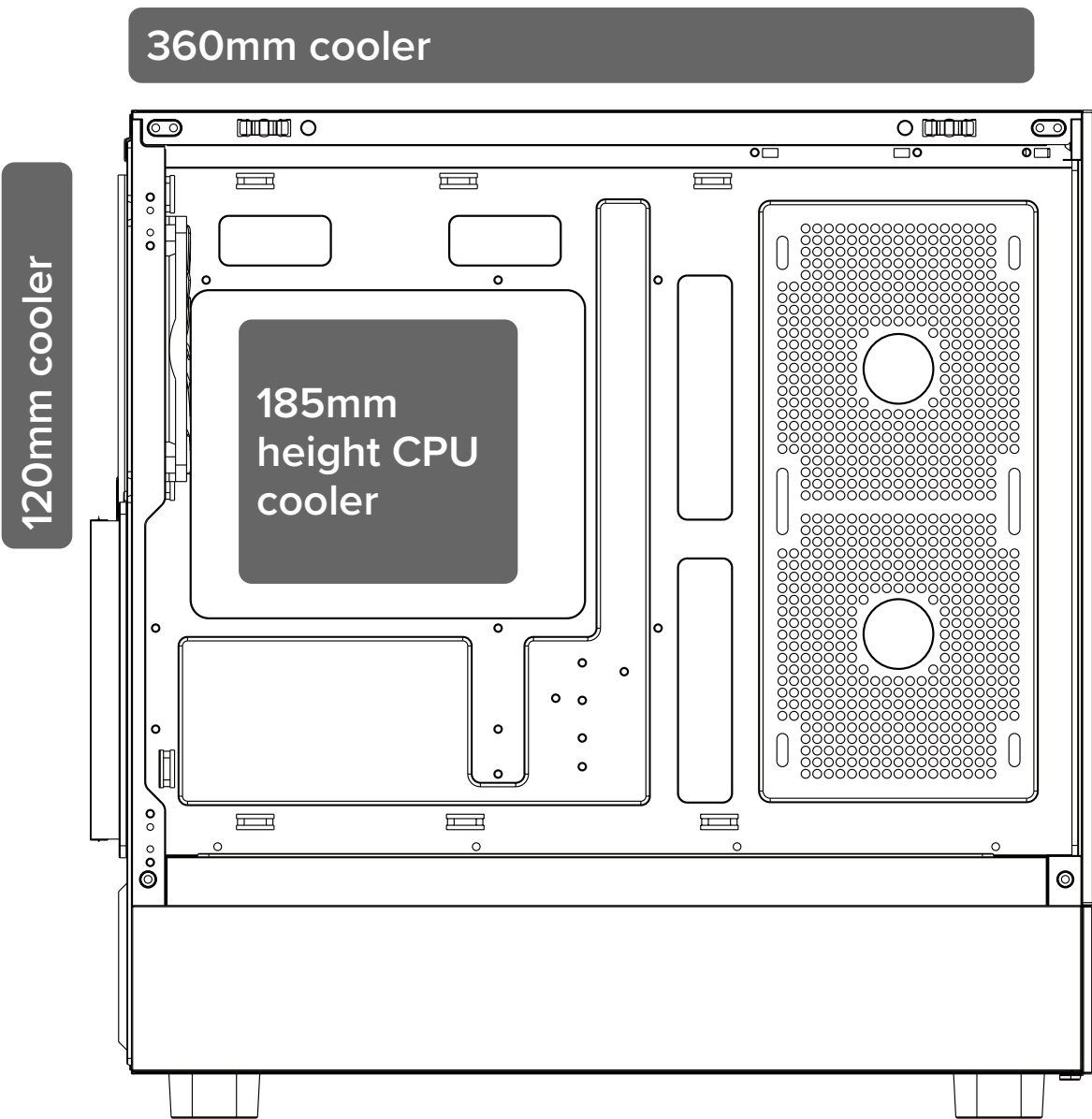
Radiator and Heatsink installation options
