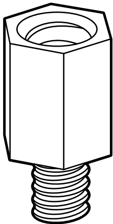
Motherboard standoffs #6-32x6.5mm x3
